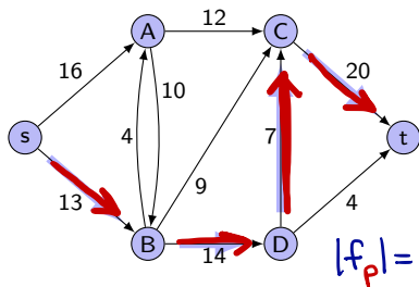
Restnetzwerk G_f |f_p| = 7 = c_f(p)
