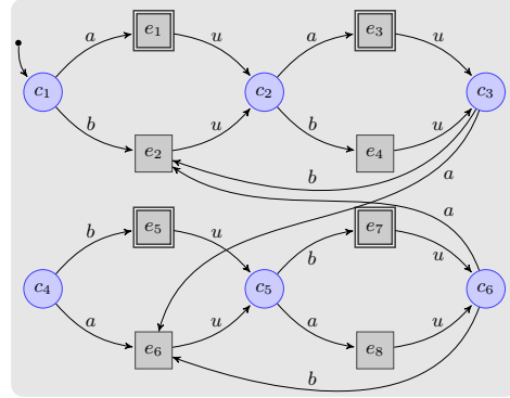
Fig. 4: A safety game winnable for the controller with finite-memory strategies with \delta_{\max} \geq 30 .
