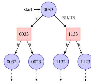
Fig. 3: A snippet of the game graph
